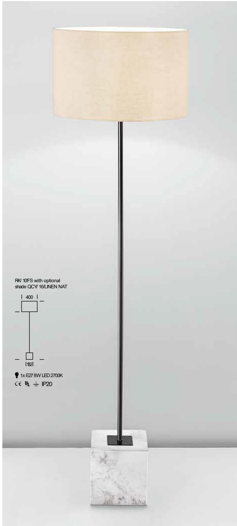
RK/ 10' TL with optional shade QCY/ 12/LINEN NAT 310 | 120 | 1x E27 7W LED 2700K CE U L IP20
